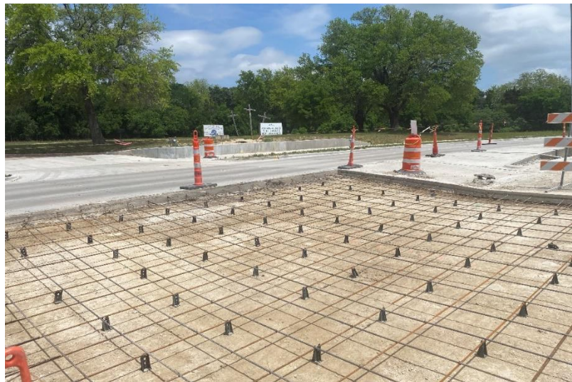
Rebar Placement at 102 E. Daniieldale Rd.
