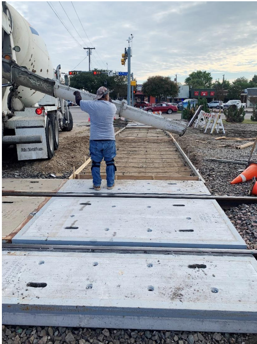
Installing sidewalk at W. Davis St. railroad crossing.
